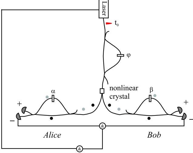
FIG. 1: Scheme of a Bell type experiment using time-bin entangled photons. Time bin qubits are prepared by passing a fs pulse through the pump interferometer. Eventually, a pair of entangled photons is created in the crystal. Alice and Bob analyze the photons using interferometers that are equally unbalanced with respect to the pump interferometer, thereby sending the amplitude in the first (gray) time bin through the long arm and the one in the second (black) through the short arm and thus undoing the transformation of the pump interferometer (in 50% of the cases).
